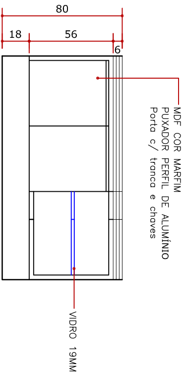
VISTA FRONTAL
